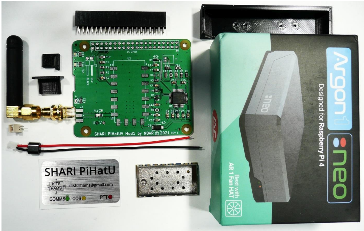
Figure 5 – SHARI PiHatU Kit Parts (Clamp-on Ferrite Core not shown)
